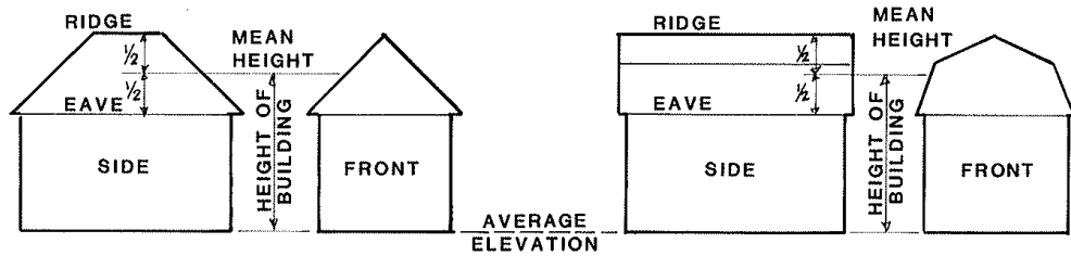
HIP ROOF
