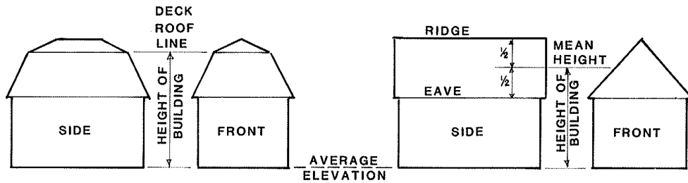
MANSARD ROOF
